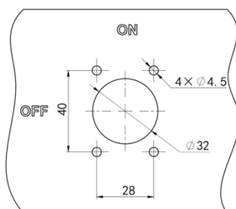
柜门安装孔尺寸 Panel drilling
